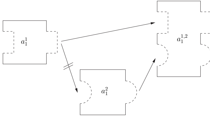
Figure 8: Agent Communication Between Overlapping Committees
