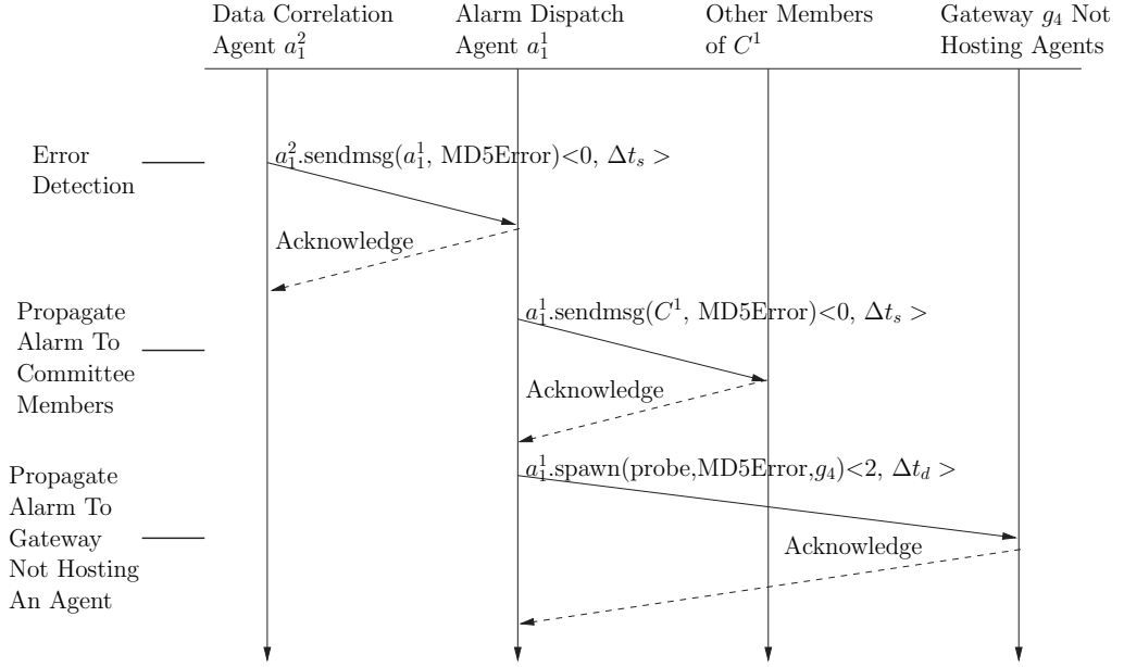
Figure 10: Propagation of Alarm Notification
