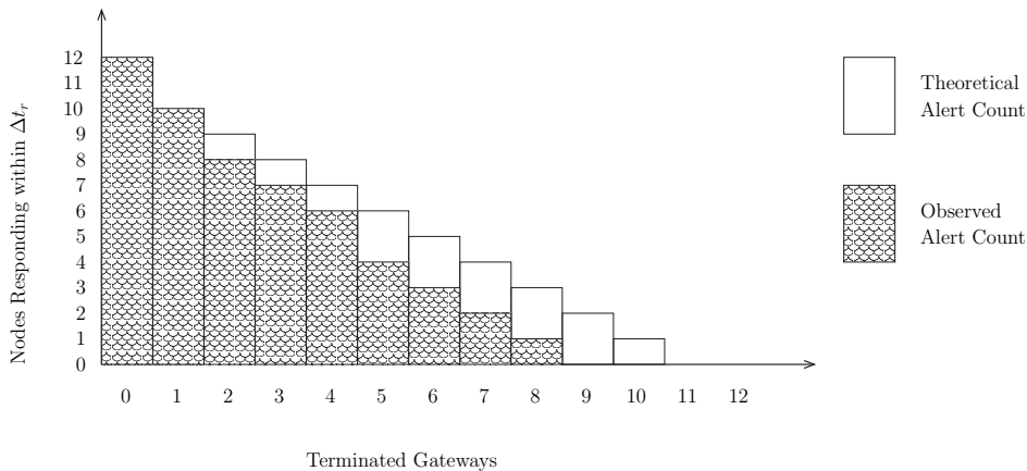
Figure 11: Agent Response in the Presence of Gateway Failure
