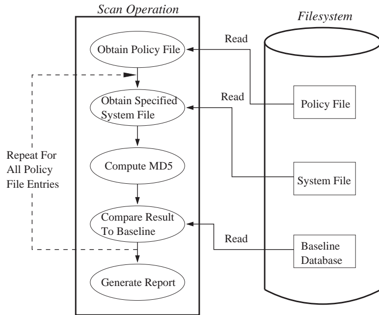
Figure 1: File Integrity Scan Operation
