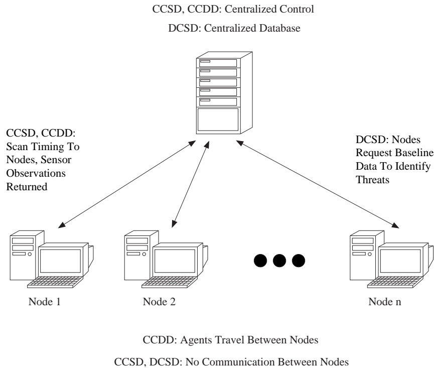
Figure 3: Control and Dispatch Strategies of IDS Architectures
