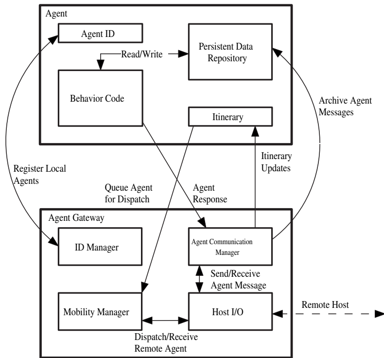
Figure 5: CONFIDANT Agent Structure [11]
