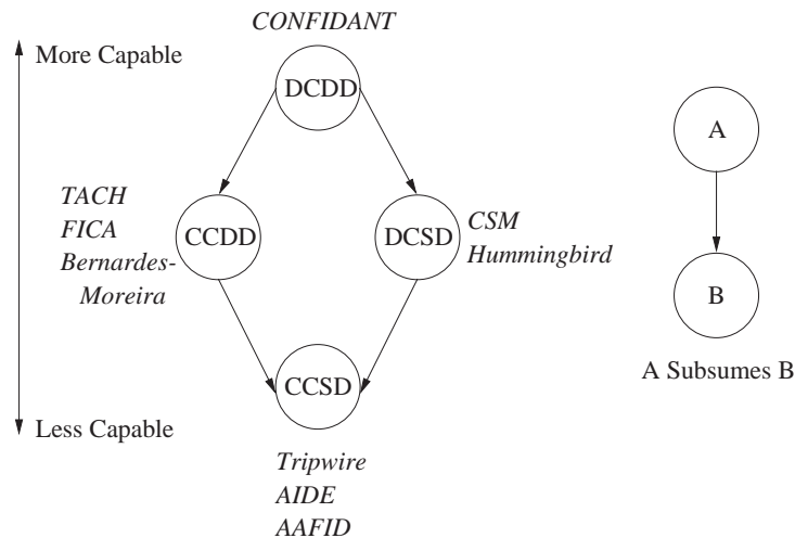
Figure 4: Hierarchy of Architecture Classes
