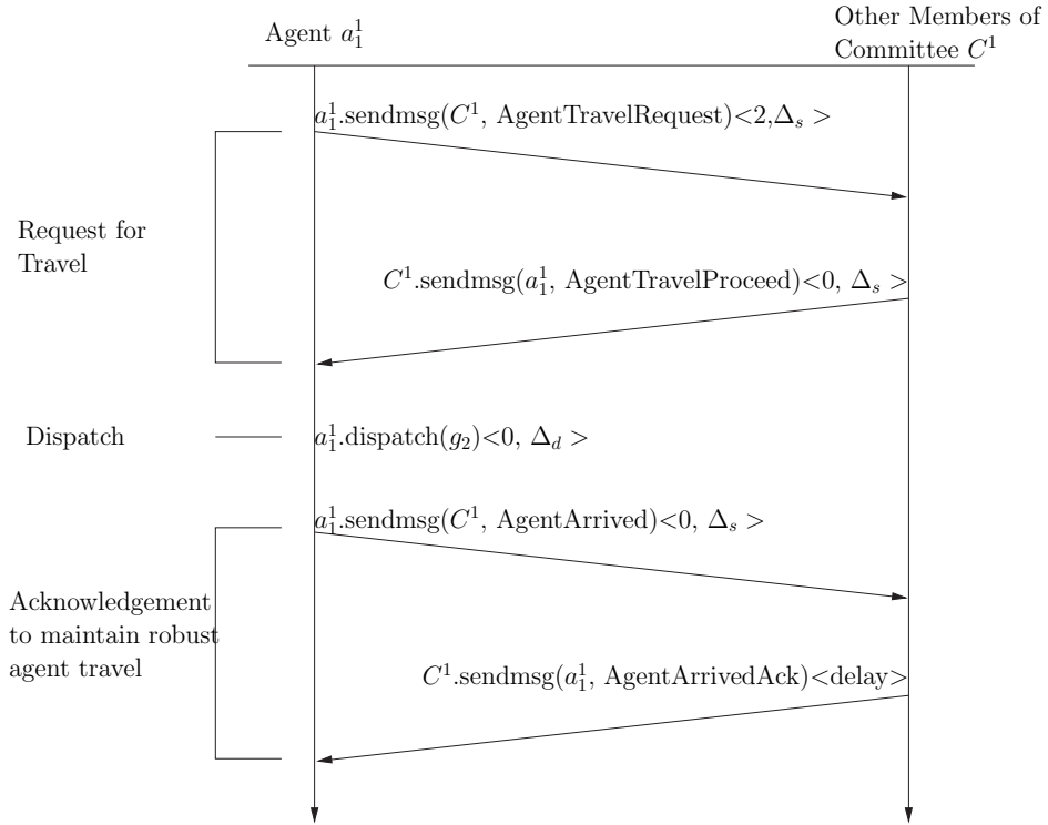
Figure 9: Dispatch and Communication Example
