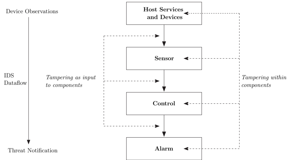
Figure 2: IDS Conceptual Architecture
